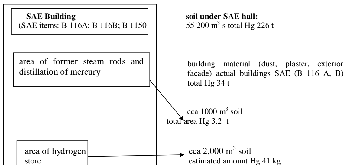
Picture 3: Specification and amounts of materials contaminated by mercury from old amalgam electrolysis (SAE). Source: Vurm, K. et al. 2001. 14
